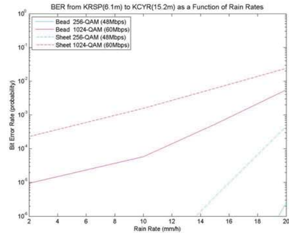
Figure represents the modeled relationship between rain rate and probability of a bit error while transmitting using both 256-QAM and 1024-QAM while rain is either sheeting or beading on the surface of the radome. The specifications of IS1's KRSP and KCYR towers were used to calculate these probabilities.
